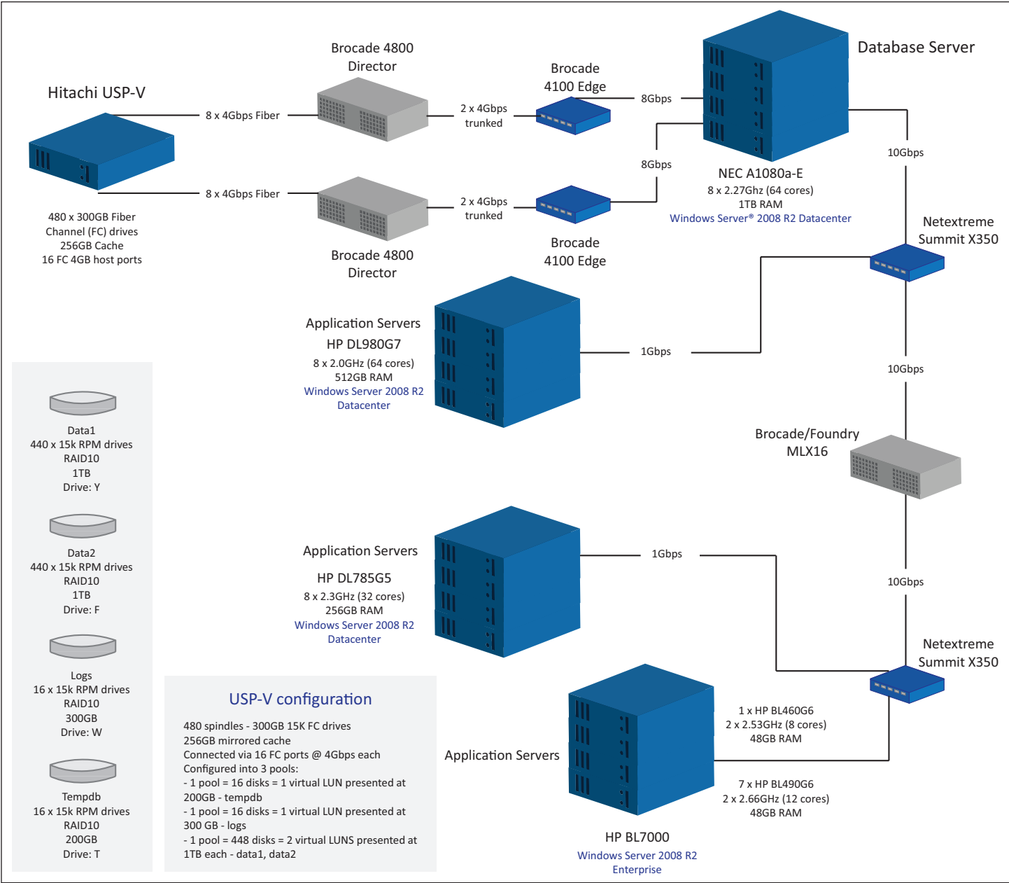
Figure 4. Hardware configuration for COB testing.
