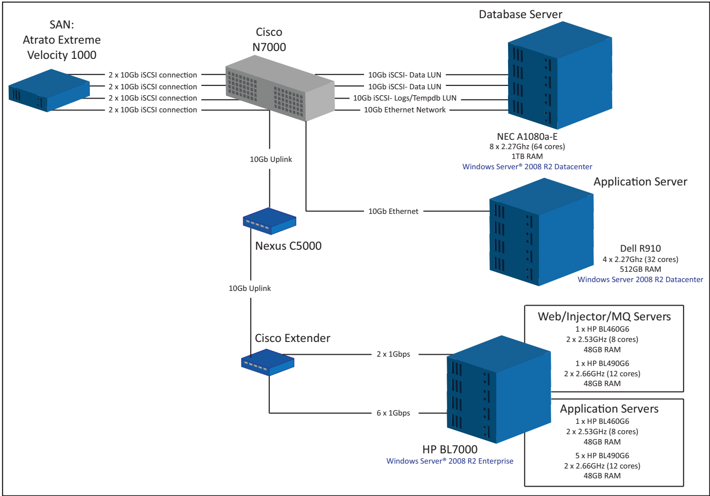
Figure 3. Online business testing configuration.
