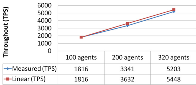
Figure 5. Scalability results.
